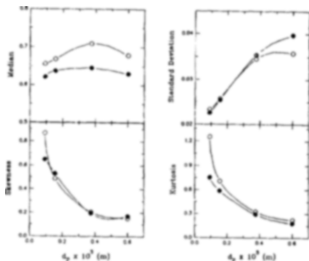
Fig. 5. Effects of d_p on median, standard deviation, skewness and kurtosis of pressure fluctuations from three phase bubble column reactors ( U_G=0.06 m/s, t=40 min, P=92 KPa, S=28 wt%, T=140^\circ\text{C} ).
